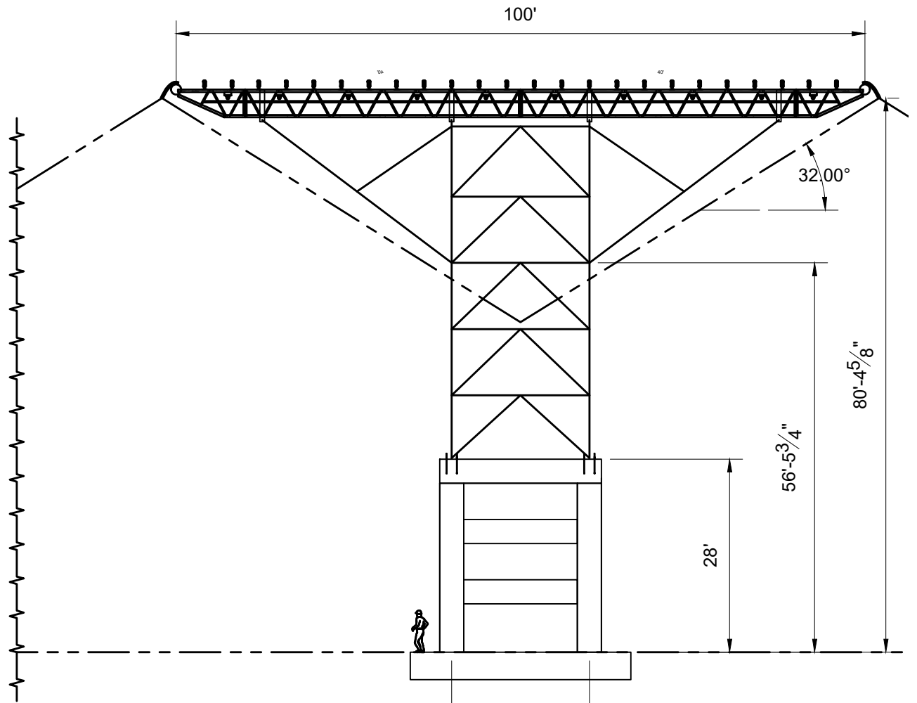
END VIEW
